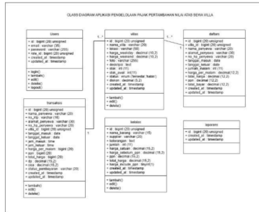
Figure 6. Class Diagram
