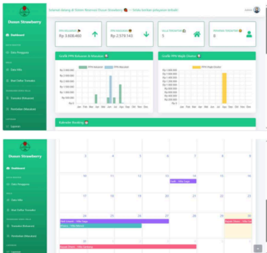
Figure 9. Dashboard page
