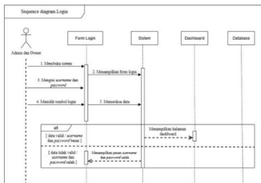
Figure 5. Login Sequence Diagram
