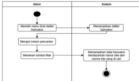
Figure 4. Activity Diagram View Transaction List (Owner)
