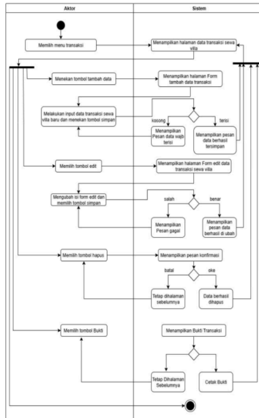
Figure 3. Activity Diagram of Villa Rental Transactions (Villa Rental Admin)
