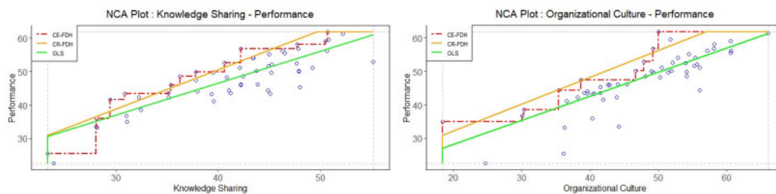
Figure 3. NCA Parameters Knowledge Sharing, Organizational Culture, Performance.
