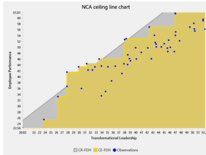
Figure 2. NCA Ceiling Chart
