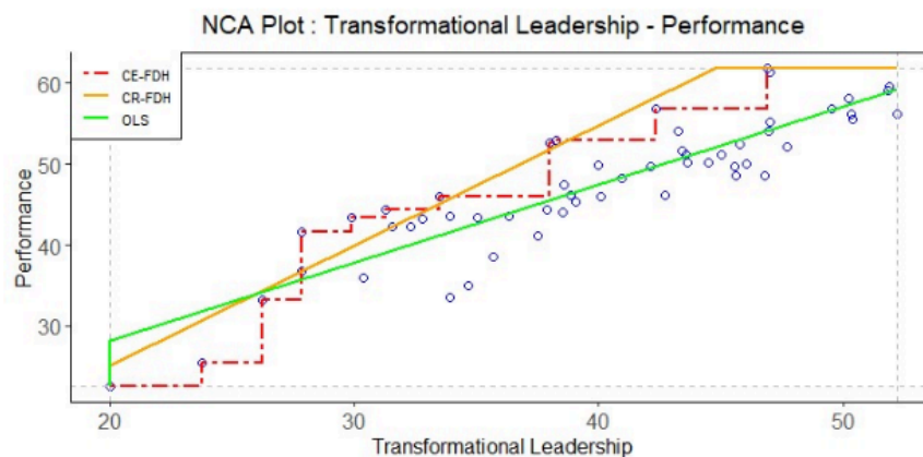
Figure 4. NCA Parameters Transformational Leadership, Performance.
