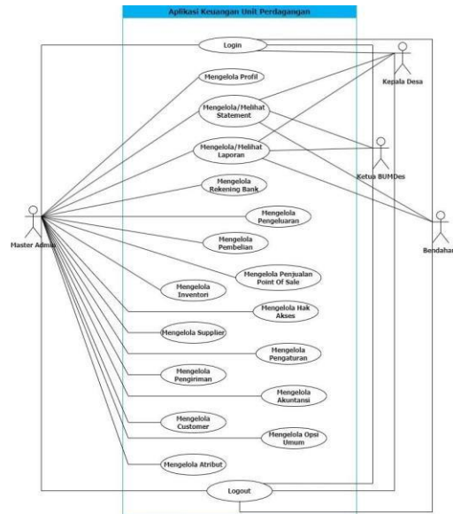
Figure 1. Usecase Diagram
