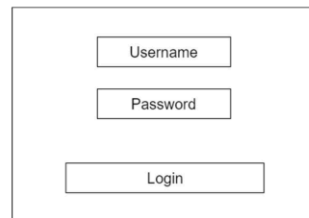
Figure 7. Login Menu
