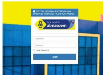
Figure 16. Login Menu
