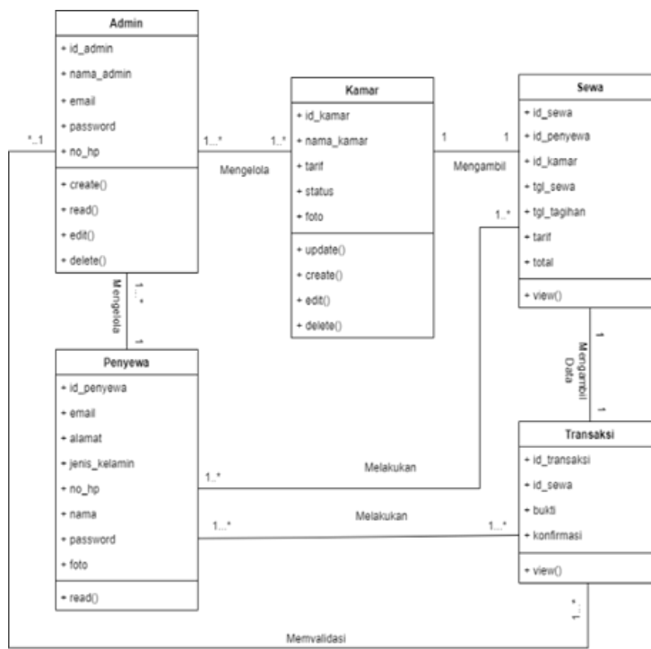
Figure 4. Class Diagram
