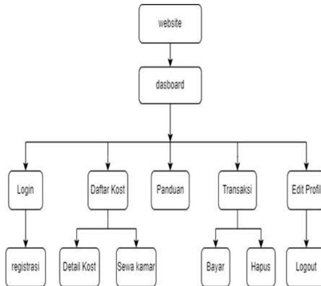
Figure 5. Interface Design
