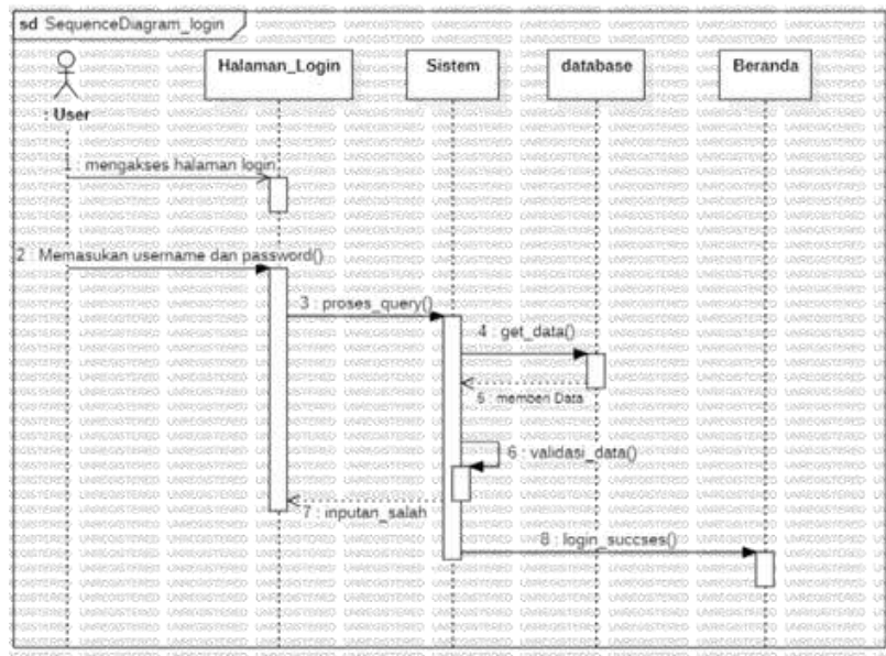
Figure 3. Sequence Diagram
