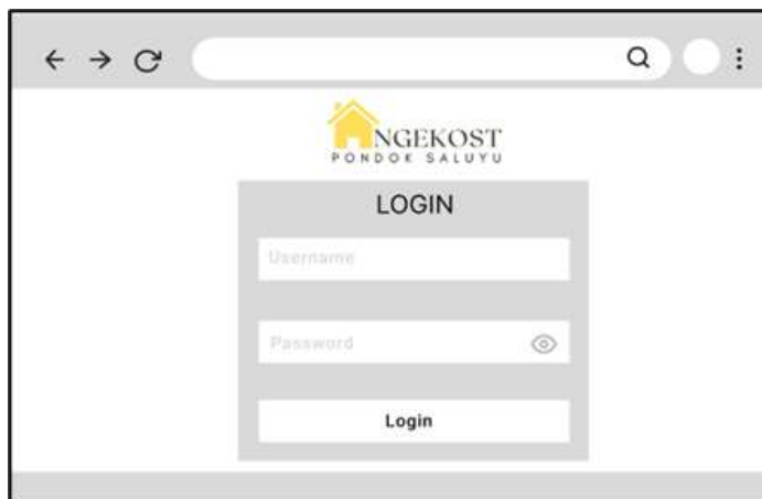
Figure 5. Interface Design
