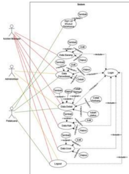
Figure 3. Usecase Diagram
