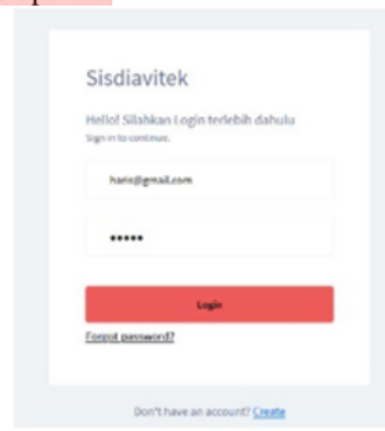
Figure 8. Page display
