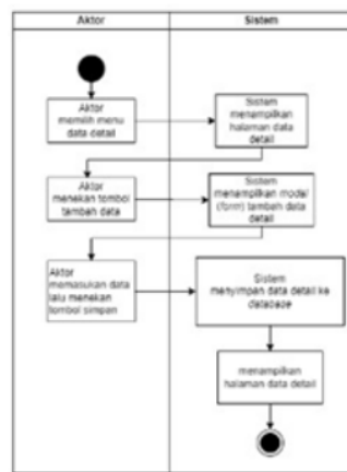
Figure 5. Activity Diagrams
