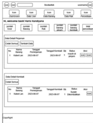
Figure 7. Interface Design
